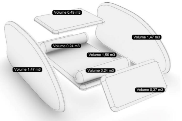
STB SIDE INFLATABLE HULL
